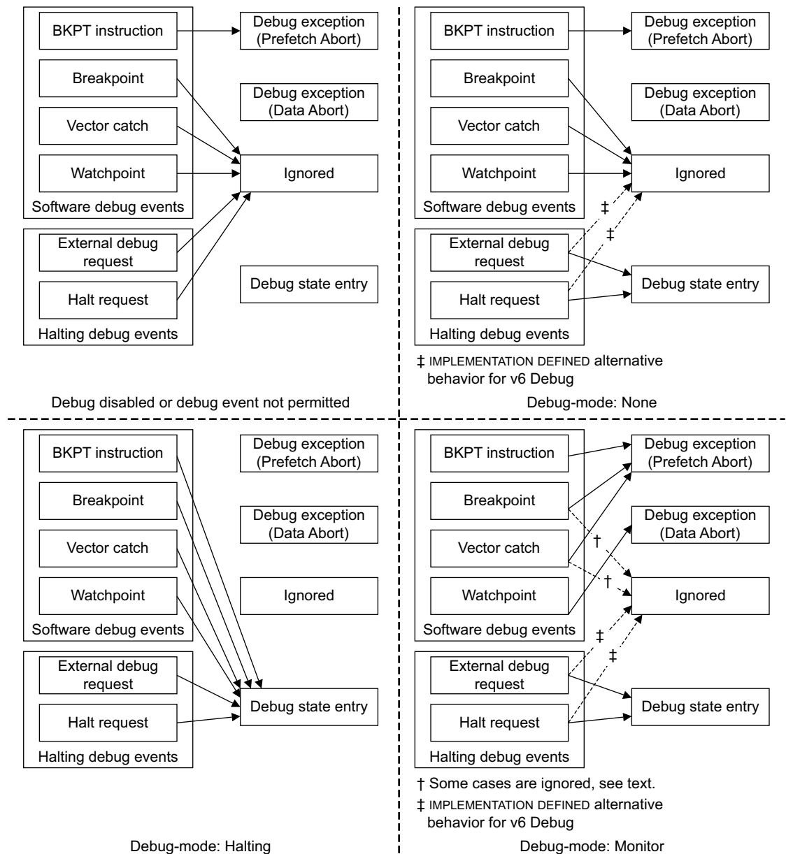
Figure D13-1 Processor behavior on debug events, for v6 Debug and v6.1 Debug
