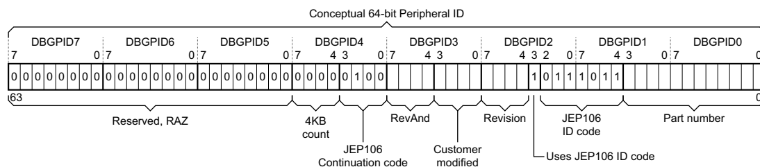
Figure C11-2 Peripheral ID fields, with values for a implementation designed by ARM
