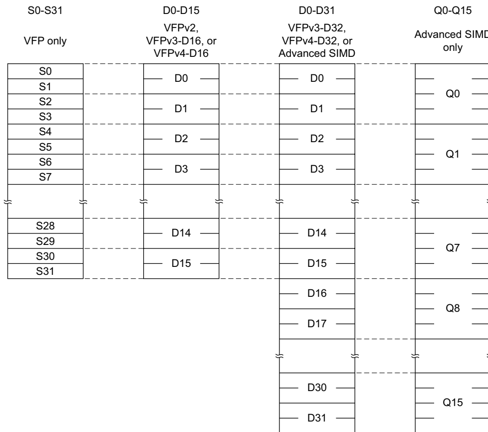
Figure A2-1 Advanced SIMD and Floating-point Extensions register set
