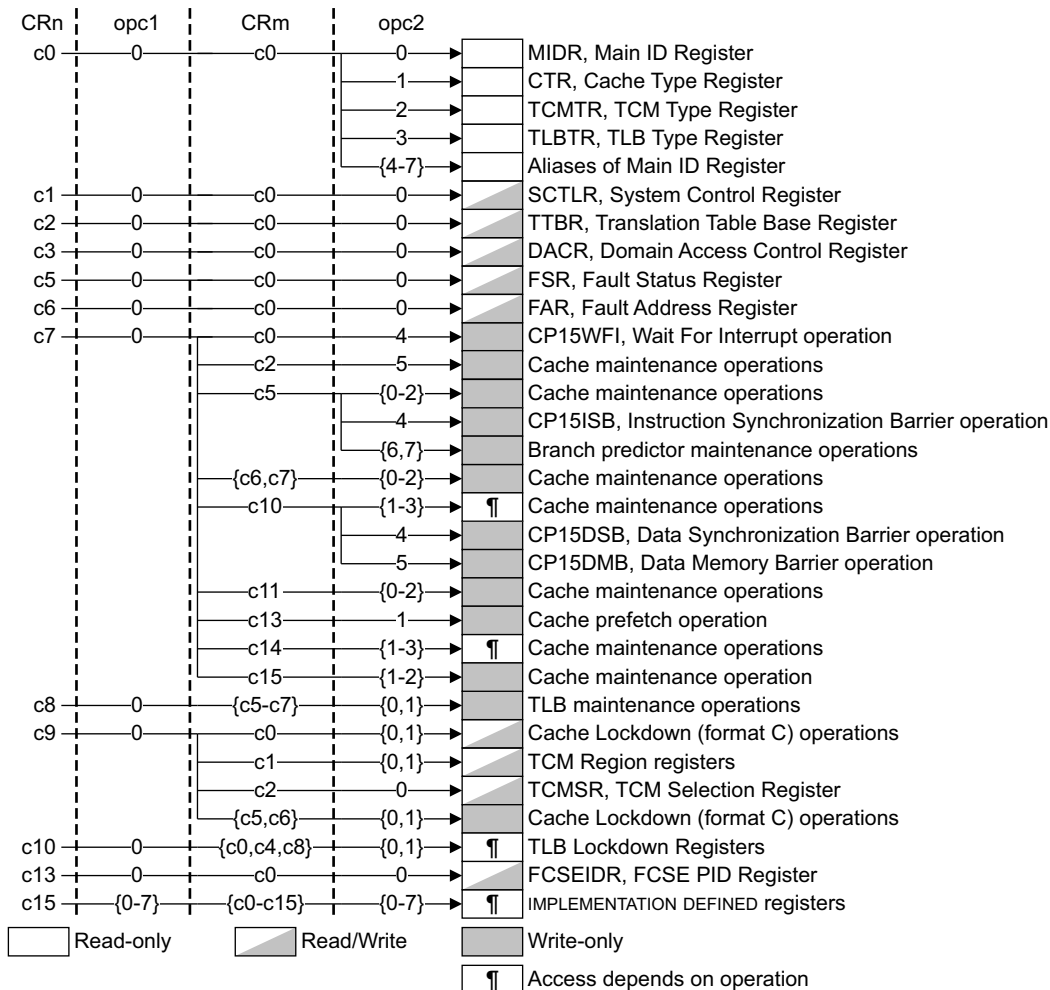
Figure D15-2 CP15 registers in a VMSAv4 or VMSAv5 implementation
