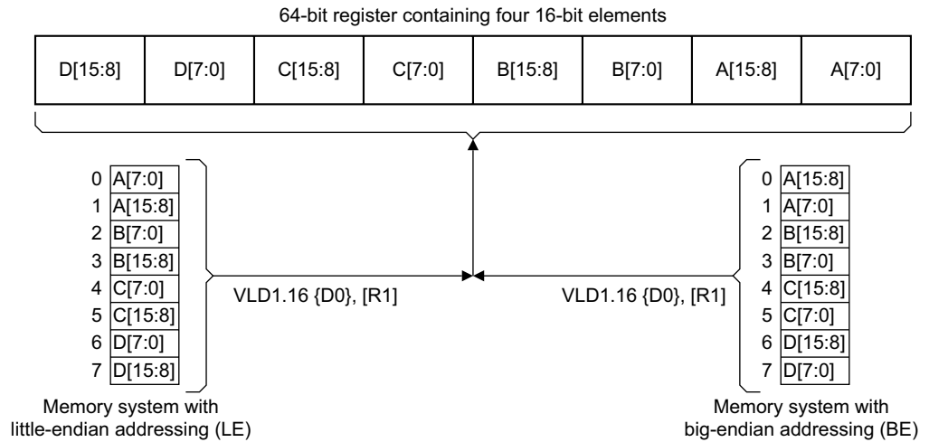
Figure A3-2 Advanced SIMD byte order example
