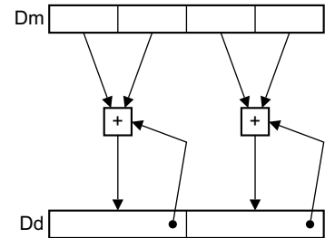
Figure A8-2 VPADAL doubleword operation for data type S16
