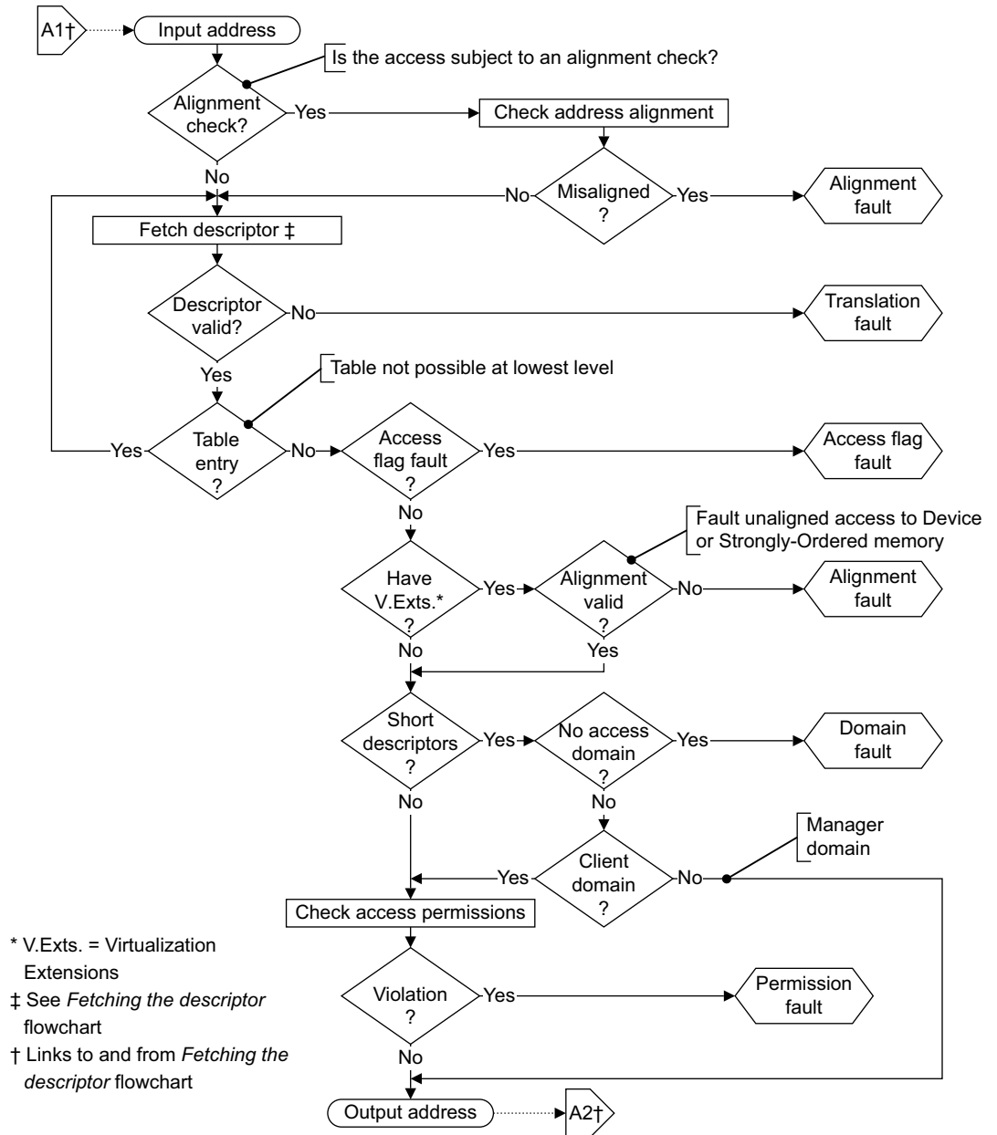
Figure B3-24 VMSA fault checking sequence
