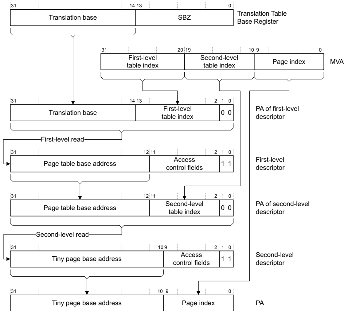
Figure D15-1 Tiny page address translation, VMSAv5 and VMSAv4 only
