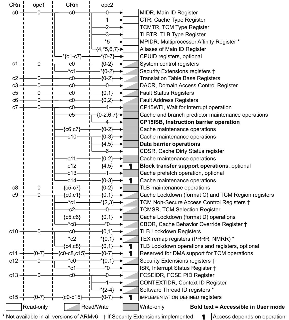
Figure D12-1 CP15 registers in a VMSAv6 implementation
