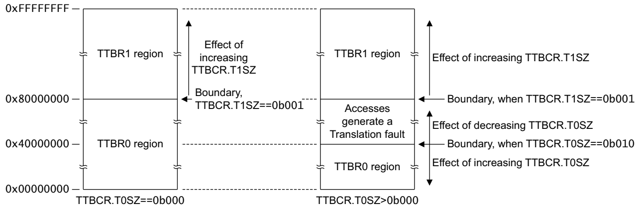
Figure B3-19 Control of TTBR boundaries, when TTBCR.T1SZ is nonzero
