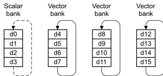
Figure D11-3 Register banks, 16 double-precision registers, VFP
