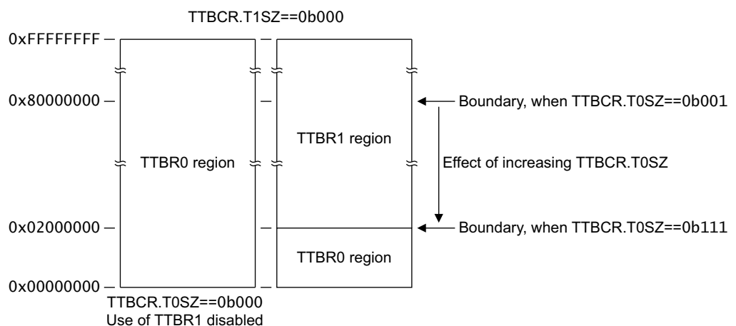
Figure B3-18 Control of TTBR boundary, when TTBCR.T1SZ is zero
