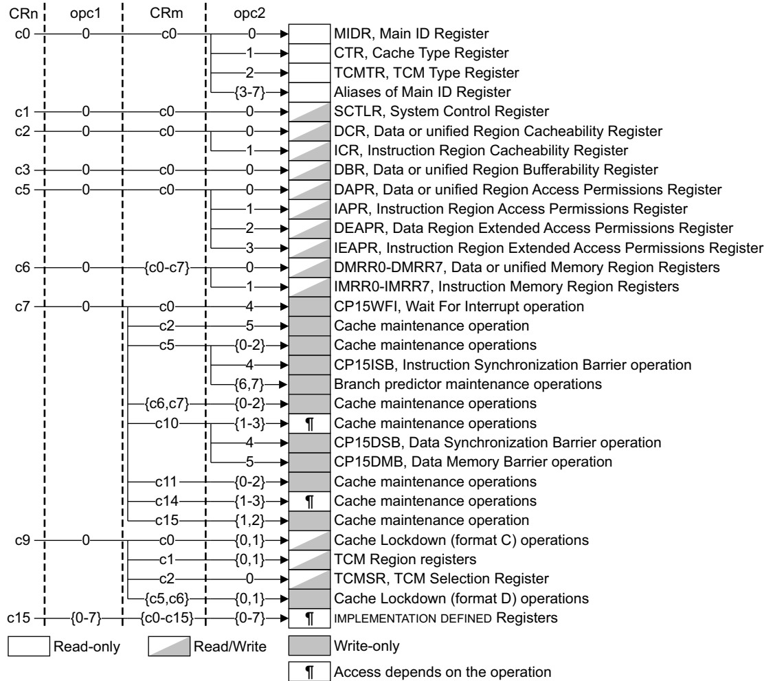
Figure D15-3 CP15 registers in a PMSAv4 or PMSAv5 implementation
