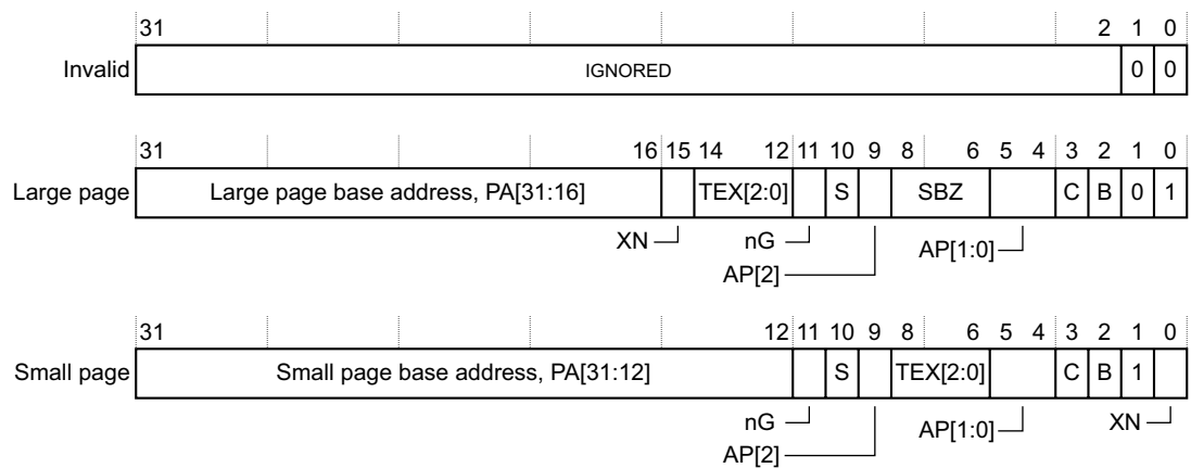
Figure B3-5 Short-descriptor second-level descriptor formats
