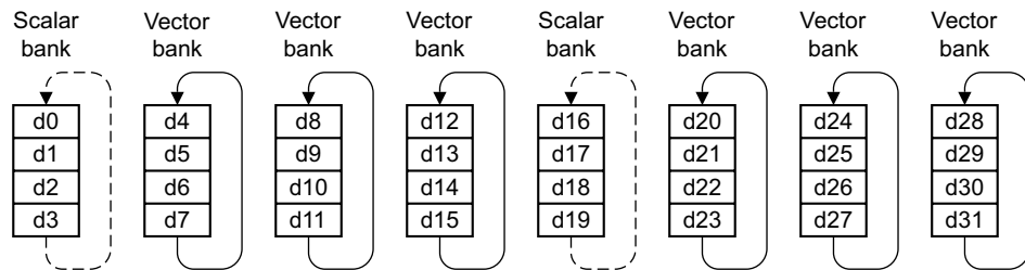
Figure D11-2 Register banks, 32 double-precision registers, VFP
