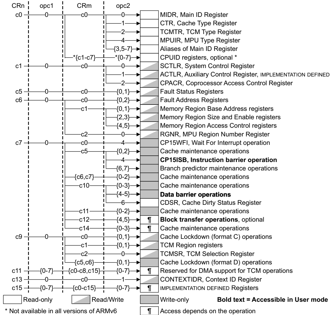
Figure D12-2 CP15 registers in an PMSAv6 implementation
