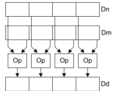
Figure A4-2 Advanced SIMD instruction operating on 64-bit registers
