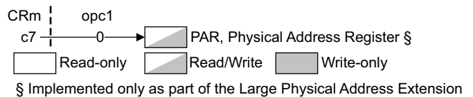
Figure B3-33 CP15 64-bit c7 registers
