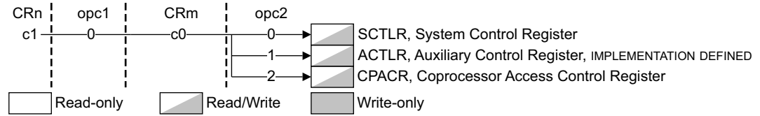
Figure B5-5 CP15 c1 registers in a PMSA implementation
