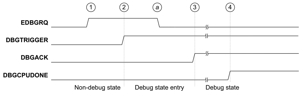
Figure D1-2 Signaling for Debug state entry on an External debug request
