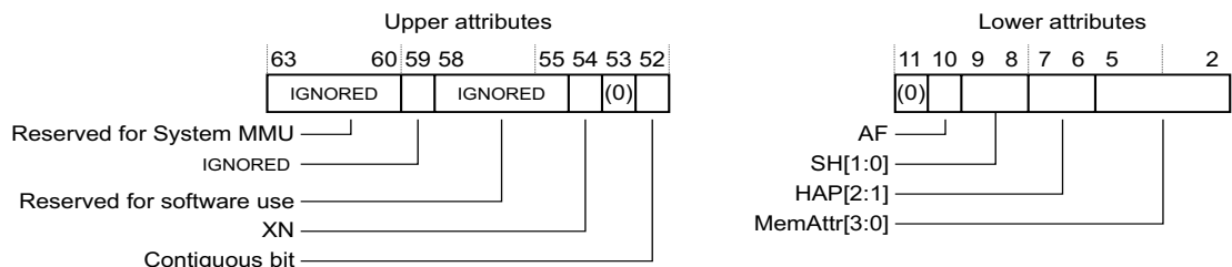
Figure B3-17 Memory attribute fields in Long-descriptor stage 2 Block and Page descriptors
