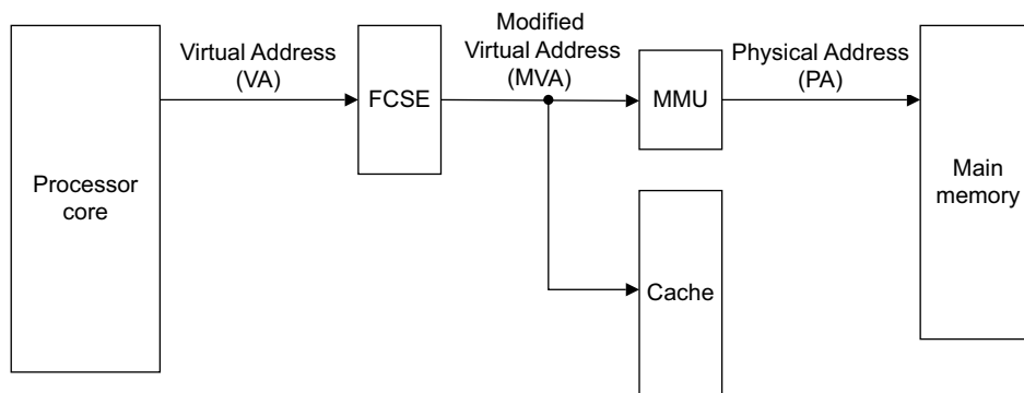
Figure D10-1 Address flow in MMU memory system with FCSE
