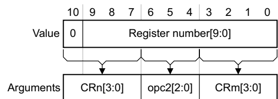
Figure C6-1 Mapping from debug register number to CP14 instruction arguments
