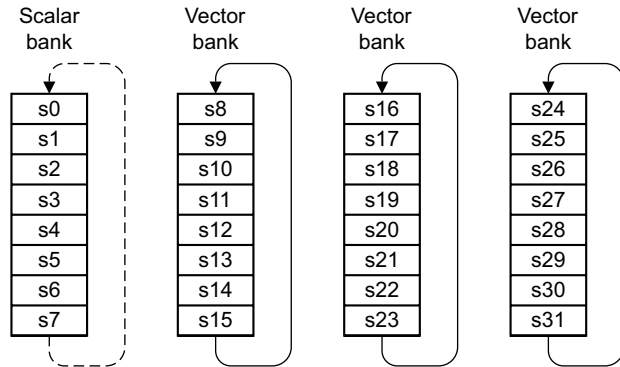
Figure D11-1 Register banks, single-precision
