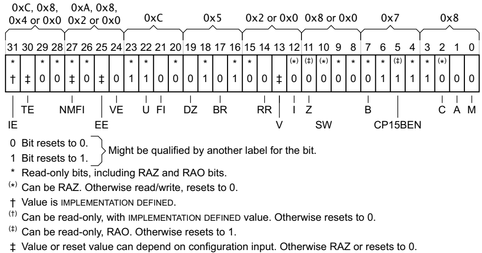
Figure B6-1 Reset value of the SCTLR, PMSAv7
