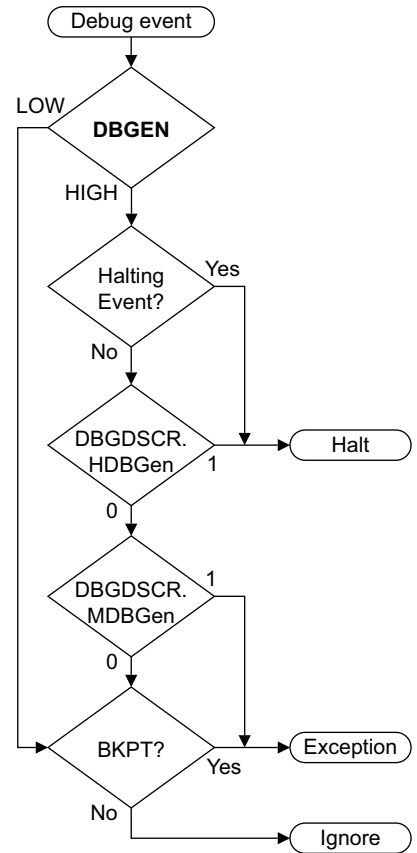
Figure C2-1 Invasive debug authentication with no Security Extensions
