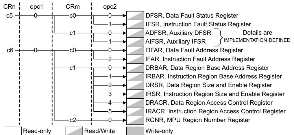
Figure B5-6 CP15 c5 and c6 registers in a PMSA implementation
