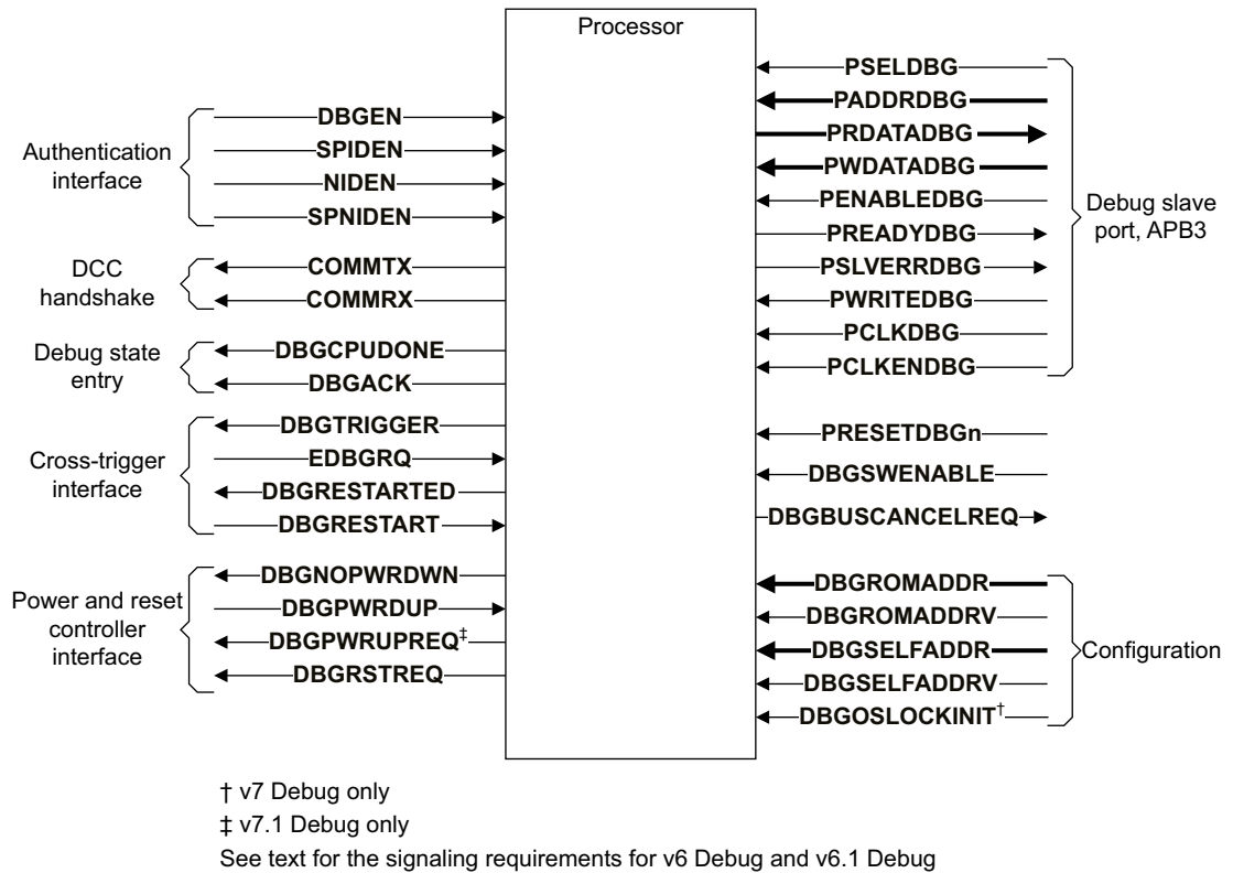
Figure D1-1 Recommended external debug interface, including APB3 slave port
