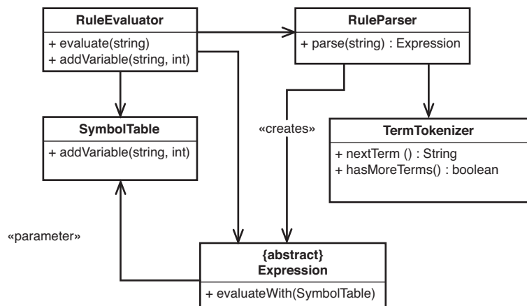
Figure 20.2 Rule classes with responsibilities separated.
