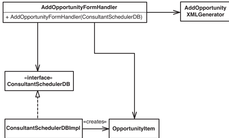
Figure 7.2 Extracting an implementer on ConsultantSchedulerDB.
