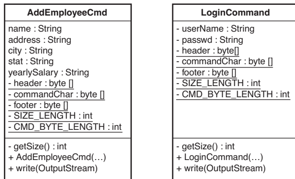
Figure 21.1 AddEmployeeCmd and LoginCommand.
