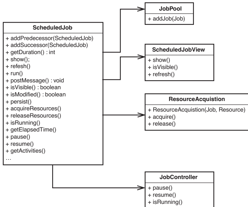
Figure 20.12 ScheduledJob with extracted classes.
