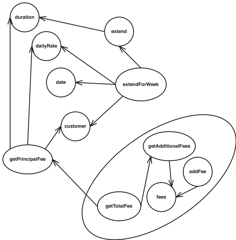
Figure 20.9 Seeing Reservation in another way.
