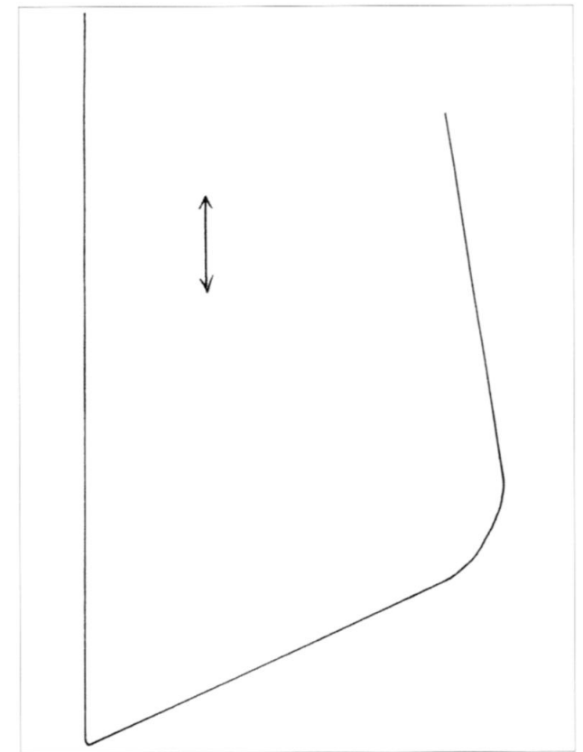
80 Pattern derived from Hedeby Fragments 11 and 76. Fragment 76 showed traces of bronze roughly 12in (30cm) above the corner. Scale 1:6
