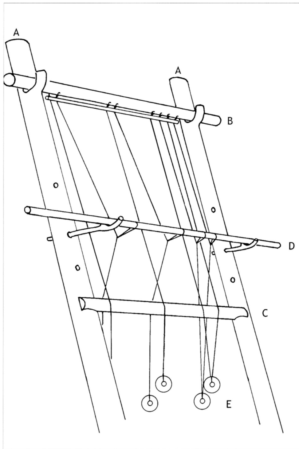
94 The warp-weighted loom: A uprights; B cloth beam; C shed rod; D heddle rod; E weights
