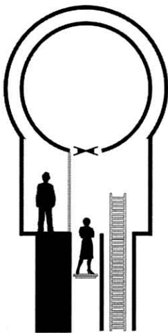
Pinnacle Dock Cross-Section
