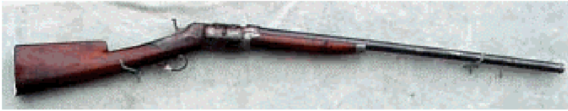
USA, Roper Revolving Shotgun, 1867-1868, Single Action, 4 shot Revolver, 12 ga, 9 lb.
