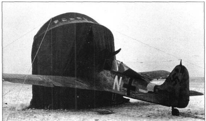
Above and right What the well-dressed Fw 190F wore in the depths of winter. Heating trollies and tents were available only for the lucky few! The latter were often reserved for aircraft undergoing in-the-field maintenance, as conditions often proved too bitter in the depths of winter for 'black men' to work outdoors for any period of time. Note that 'White N' has had a toned down cross applied to its fuselage, although its overall effect is spoiled somewhat by the full-colour Staffel markings
