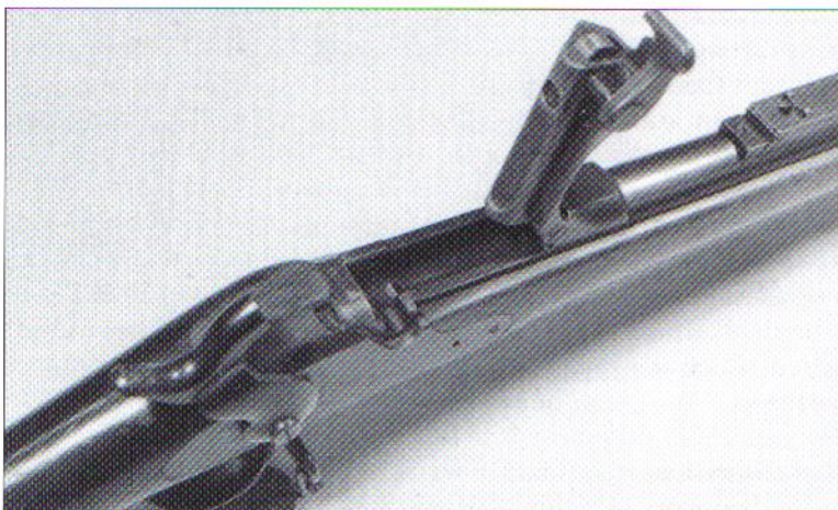
The black infantry regiments were armed with the breech-loading Springfield 'Trapdoor' rifle by 1873. A detail showing the rising breech-block loading mechanism which gave the weapon its 'Trapdoor' nick-name. (Courtesy of the Ministry of Defence Pattern Room)
