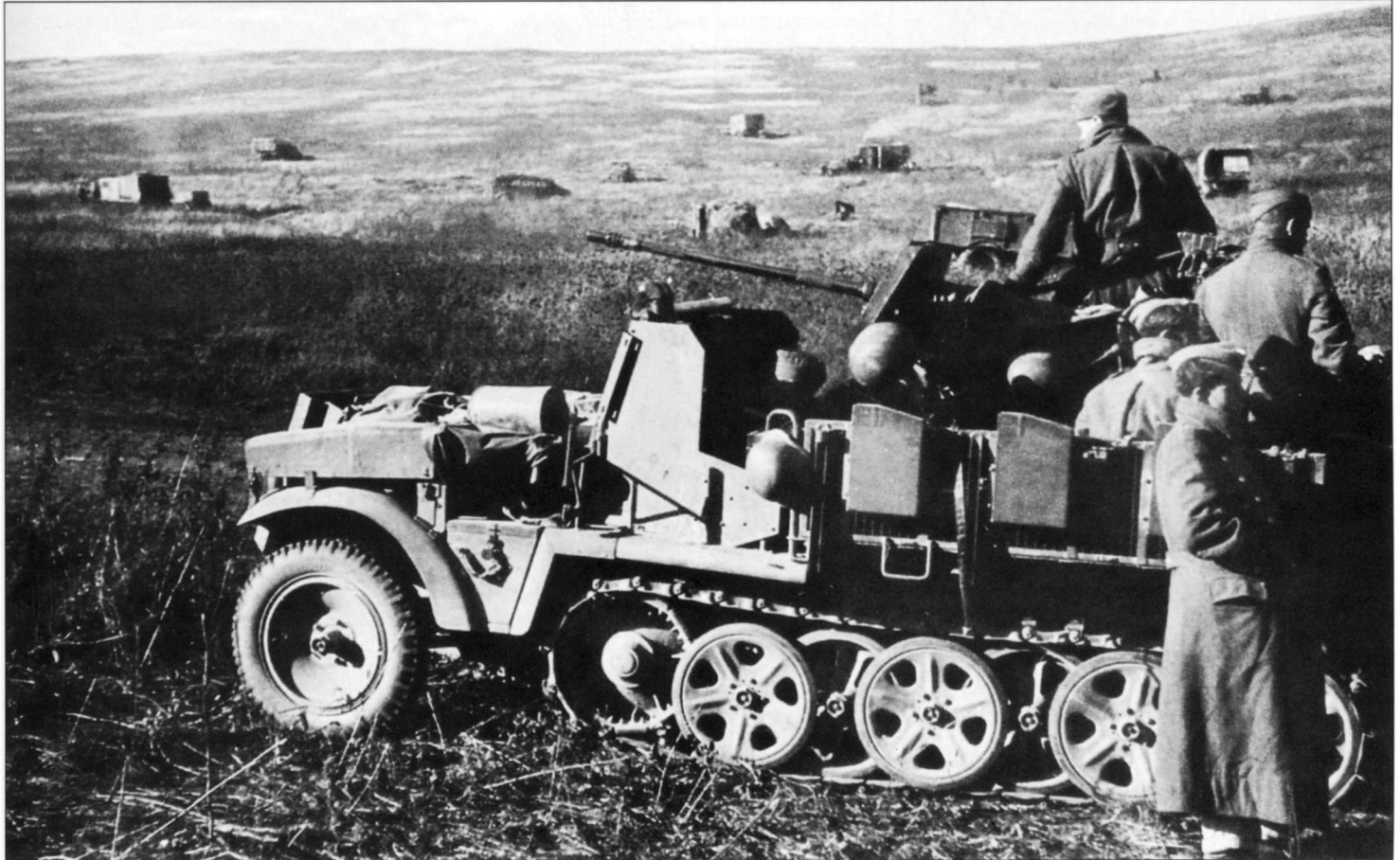
A Sd.Kfz. 10/4 with a partially armored cab and armored shield in front of the engine guards a unit's assembly area on the eastern Ukrainian steppes in the early spring of 1942. Note the binocular-type telescope installed in the driver position — a very rare piece of equipment for such vehicles, especially in this location.
