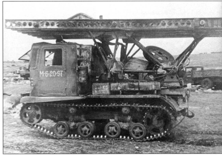
One of the rarer vehicles — the BM-13-16 missile launcher installed on the STZ-5 tractor chassis. The "Stalin organ", which was usually installed on a truck chassis or obsolete combat vehicle, could launch 82mm (M-8) or 132mm (M-13) missiles with, respectively, 3-kg and 18.5-kg warheads at ranges of 5.5 km (3.4 miles) and 8.5 km (5.3 miles). This vehicle was captured by the Germans when they eliminated the Soviet troops in the deadly cauldron east of Kharkov. It may belong to the 206th or 110th Independent Guards Rocket Squadron. Note the unit markings painted on the door of the cab.
