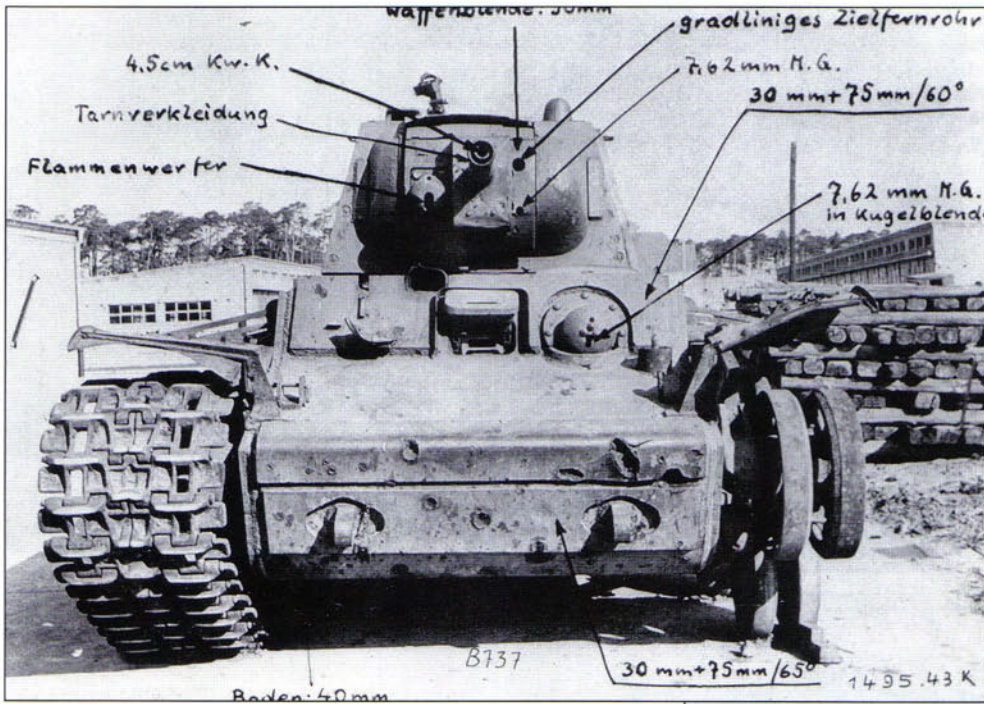
This German intelligence photo shows a captured KV-8 flamethrower tank. This front view clearly shows the 45mm gun within a thin sheet metal barrel. The flamethrower housing can be seen low to the left of this.
