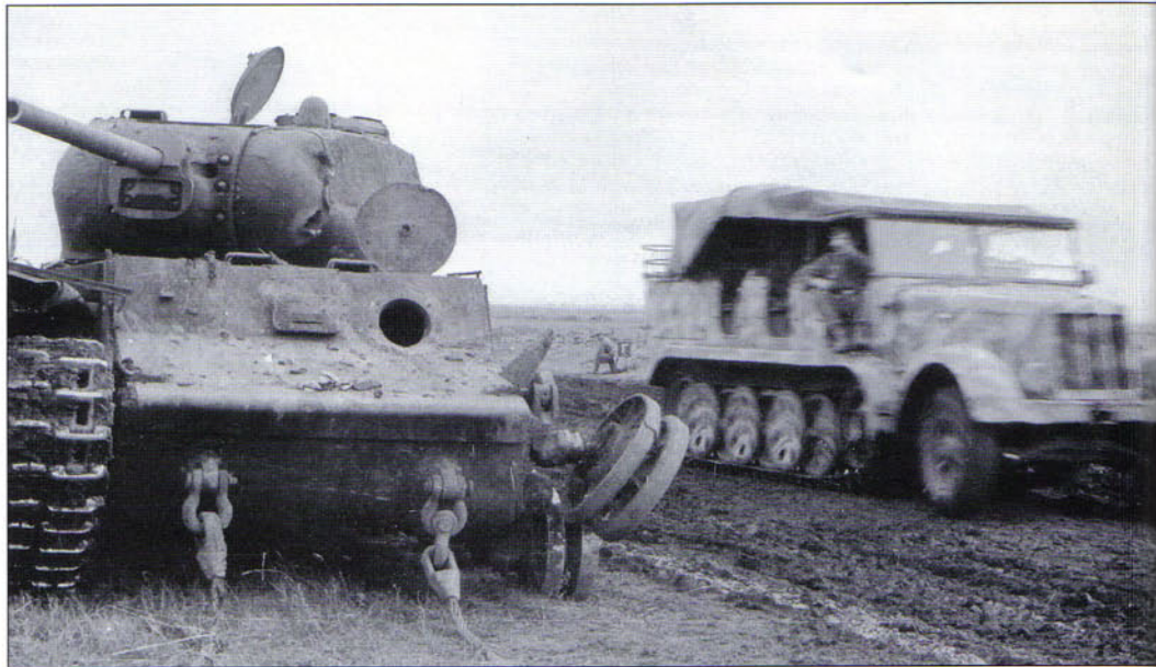
A KV-1S knocked out during the summer 1943 Kursk battles as a German SdKfz 7 half track passes by. The tank has been hit at least twice on the front side of the turret, while another shot has knocked off the hull machine gun and ripped off the front idler wheel. From the tow cables in front of the tank, some effort was made to tow it away before it was finally abandoned.
