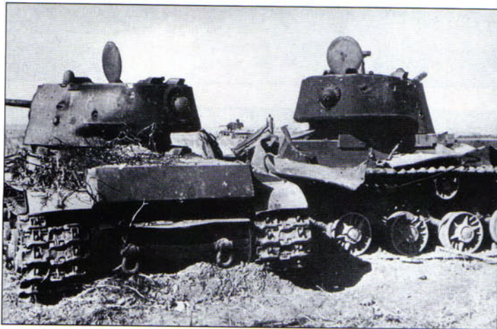
A pair of KV-1 tanks knocked out in the summer of 1942. The tank to the left has the uparmored cast turret, evident by the ring around the rear turret machine gun. The vehicle to the right has the original cast turret configuration.
