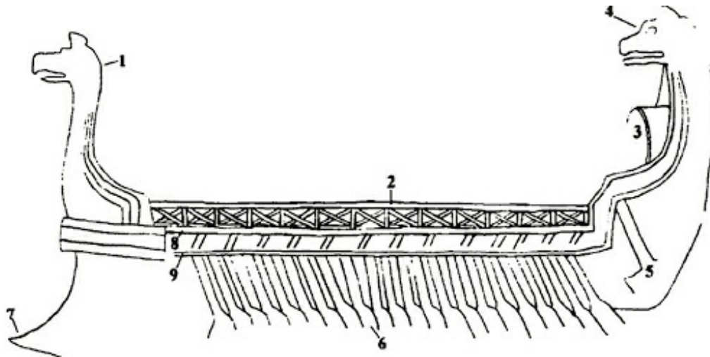
Diagram of the wine ship. (Drawing by Andrea Salimbeti ex Royal) 1. Zoomorphic head 2. Screen 3. Stern structure 4. Zoomorphic head 5. Quarter rudder 6. Oars 7. Ram 8. Sheerwale 9. Wale, outboard gangway
