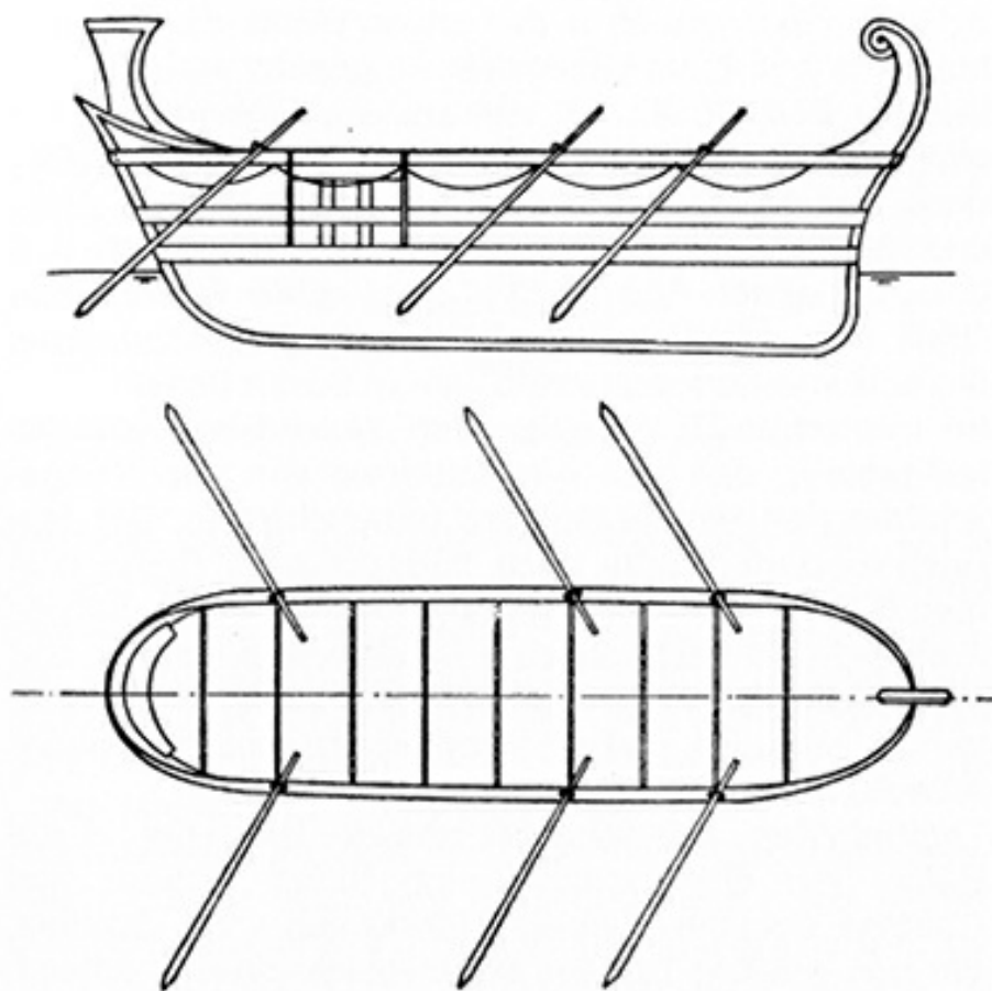
Reconstruction of a hippagus , third century AD. (Drawing by Andrea Salimbeti ex Viereck)
