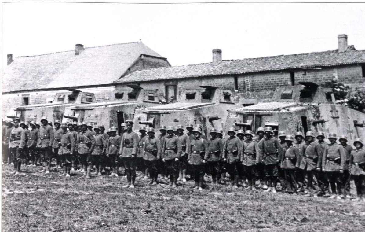
ABOVE Abteilung 2 is seen here in the summer of 1918 during training near Reims. The tanks are, from left to right, "Wotan" (563), "Hagen" (528), "Siegfried" (525), and "Schnuck" (504). (NARA)
