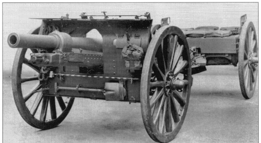
The Mark 4 18-pdr field gun, a much improved design with a maximum range of 9,300 yards (5 miles). Very few of these guns reached the BEF before the Armistice. (Author's collection)
