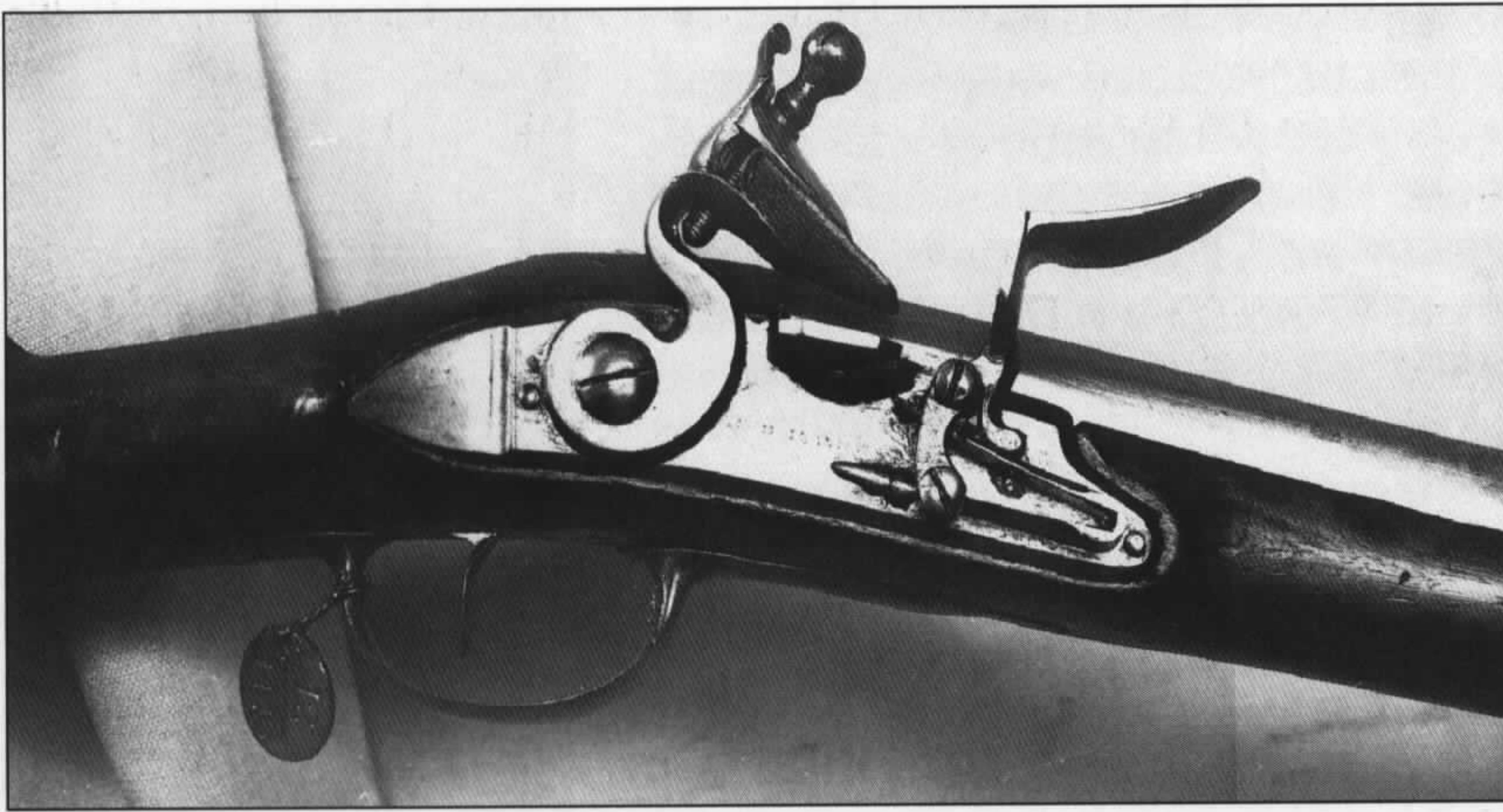
Lock detail of the 1717 Model army musket. Note the distinctive bridle connecting the frizzen spring screw with the frizzen screw. The only known mint example is at the Tower of London. Another was at Dresden but vanished during the Second World War. (Photo courtesy C. Ariès, Nantes)
