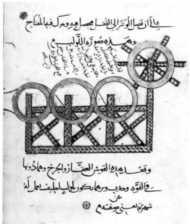
The ziyar and its loading mechanism. This was a large mounted crossbow reinforced by a wooden frame with taut ropes giving added strength to the arms of the bow. The bolt emerged from a small 'gateway' in the centre of the weapon. From al Tarsusi's late 12th-century military treatise (Ms. Hunt. 264, Bodleian Lib., Oxford) See Plate C1.
