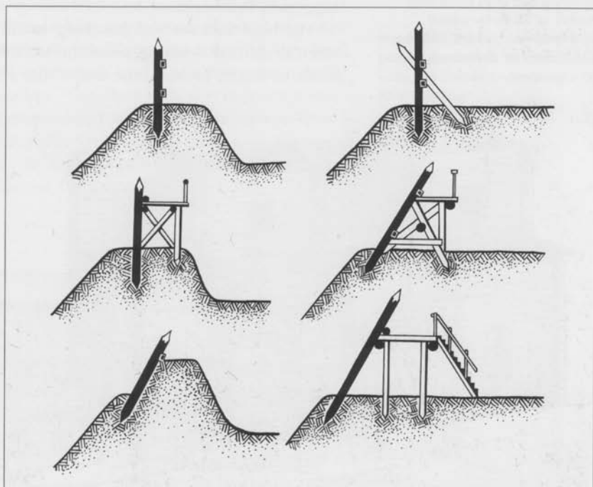
Sections through reconstructions of the various configurations of tyñ or timber paling wall as used from the 13th to 16th C, from the simplest stockade, through the more elaborate ostrog sloping types, to the incorporation of scaffolding-framed inner works. (O.V.Tymkina)
