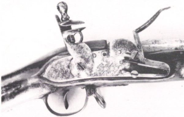
Lock of the 1809 musket as manufactured at Potsdam.
