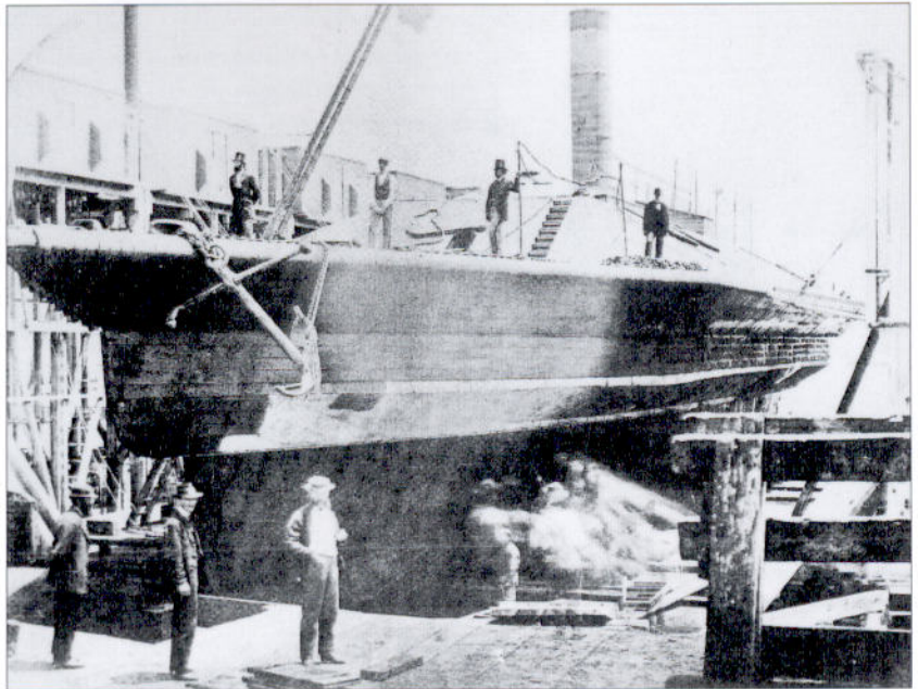
This rare view of the Atlanta in dry dock shows the shape of her lower hull, and the relatively deep draft of a typical early- or mid-war ironclad. The lack of cladding on the underside of the hull led to irreparable rotting in both the North Carolina and the Baltic . (National Archives, Washington)
