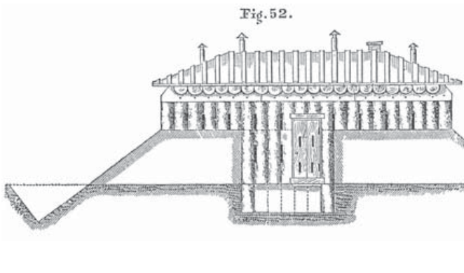
This plan and elevation of a blockhouse of single thickness, and showing the entrance protected by a gallery, was published in Mahan's An Elementary Course of Military Engineering in 1865. (Author's collection)
