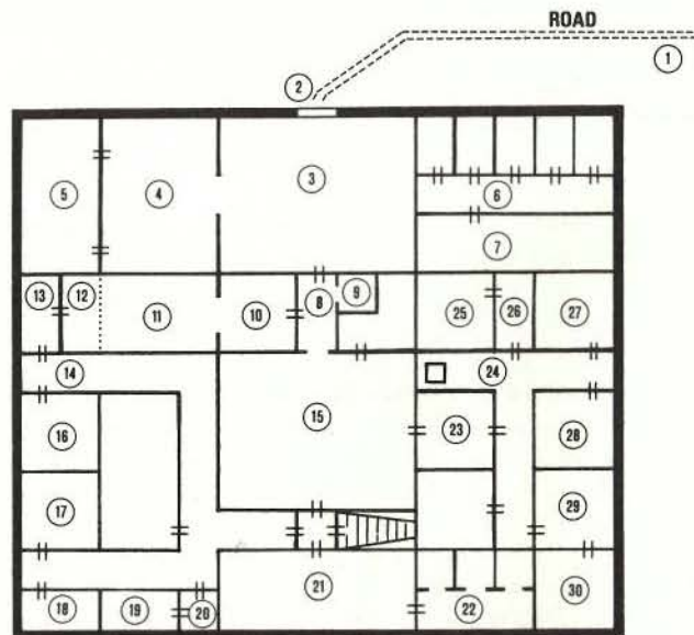
MAIN FLOOR
